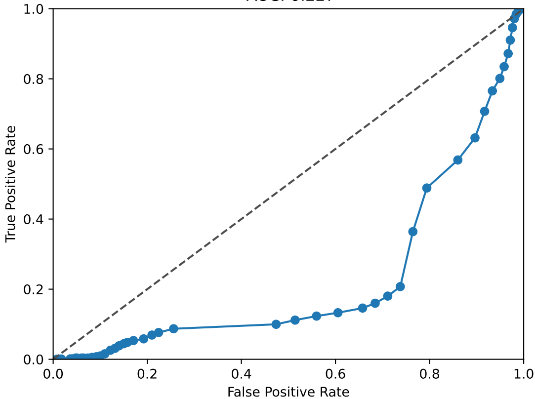
NFIX ROC Curve AUC: 0.227
