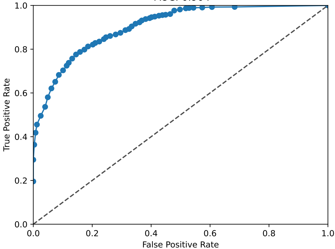
RORA_RORB ROC Curve AUC: 0.904
