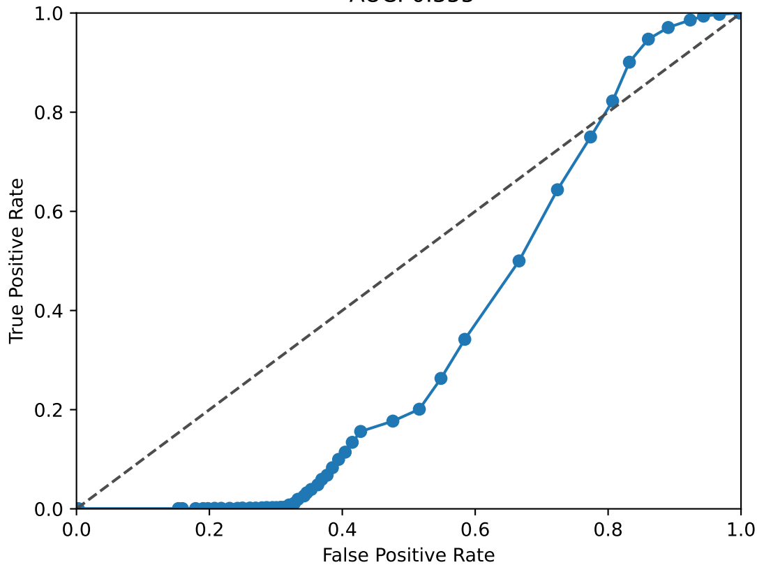
TCF7L2 ROC Curve AUC: 0.355
