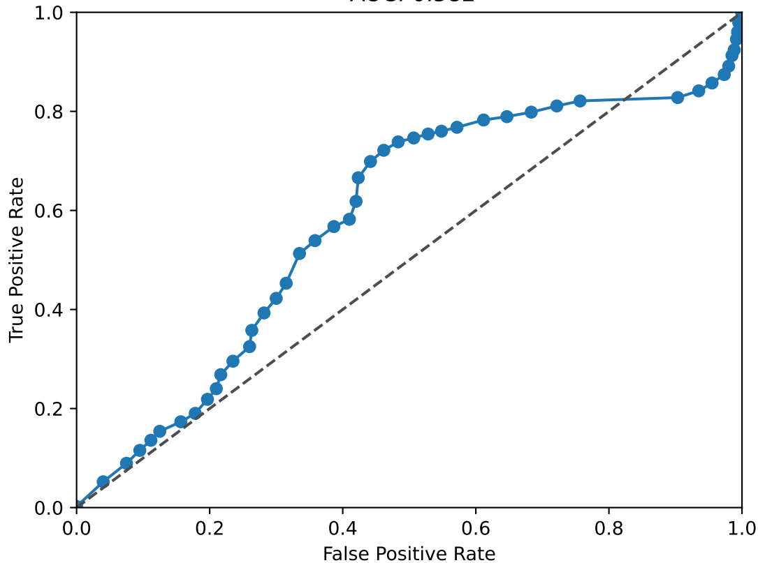
EGR1 ROC Curve AUC: 0.582
