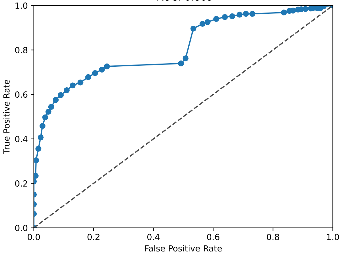
JUNB ROC Curve AUC: 0.809
