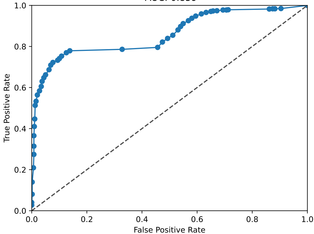
JUN ROC Curve AUC: 0.859
