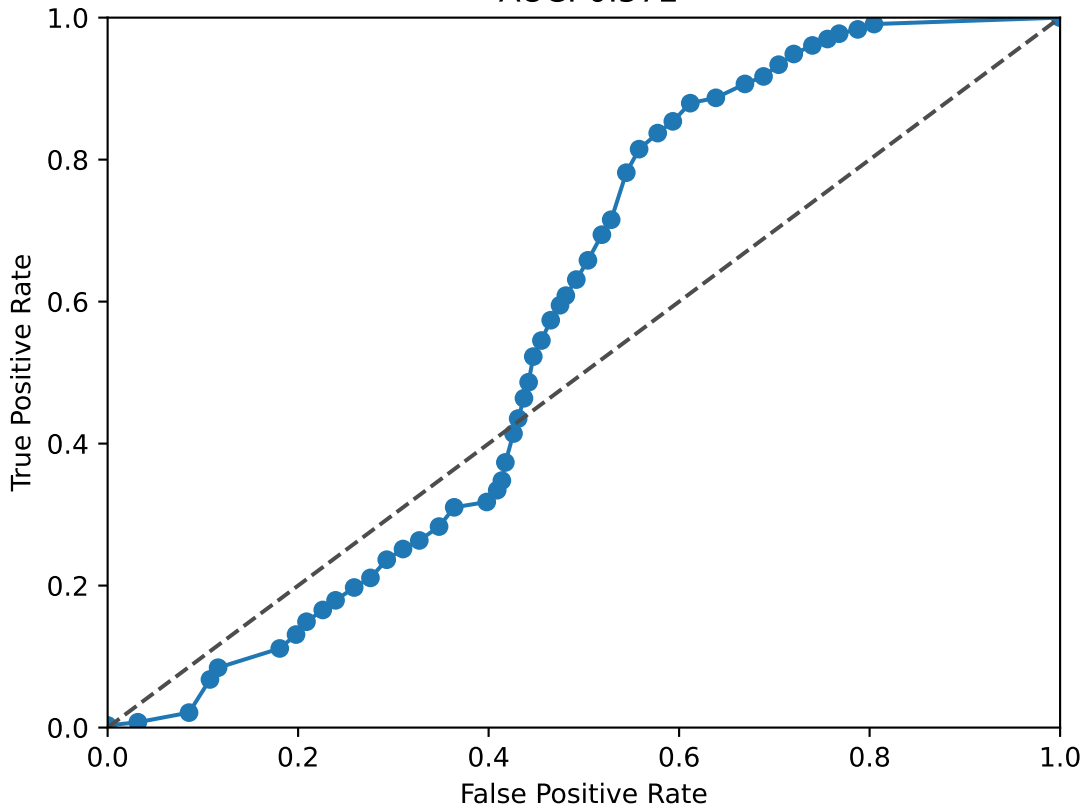
NFIA ROC Curve AUC: 0.572
