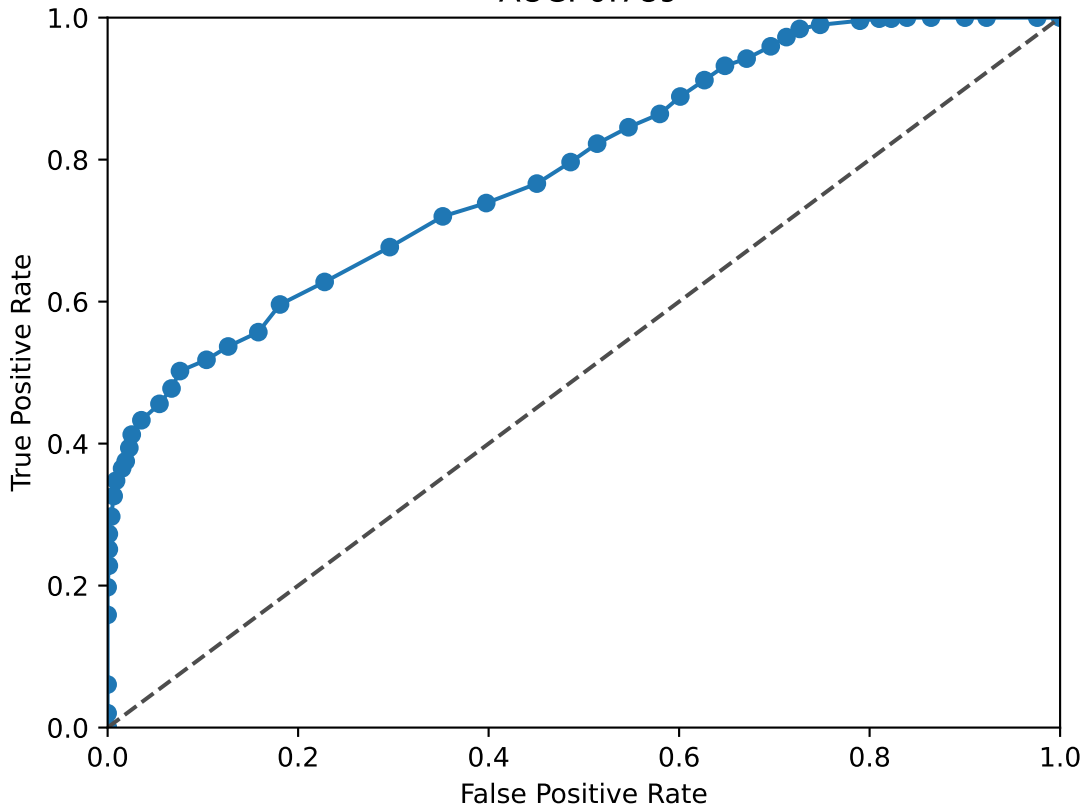
NFIB ROC Curve AUC: 0.789
