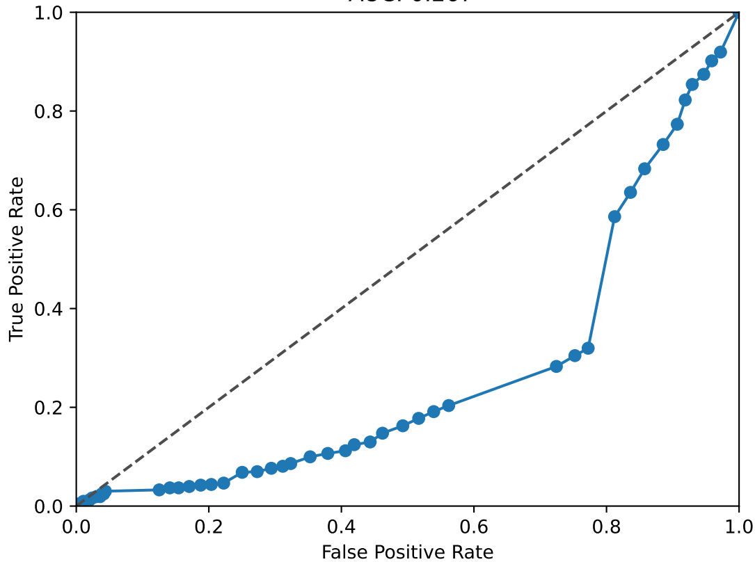
REST ROC Curve AUC: 0.267
