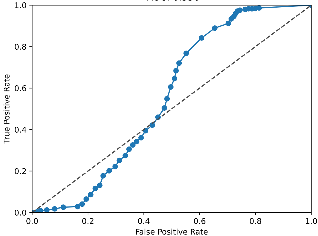
STAT2 ROC Curve AUC: 0.556
