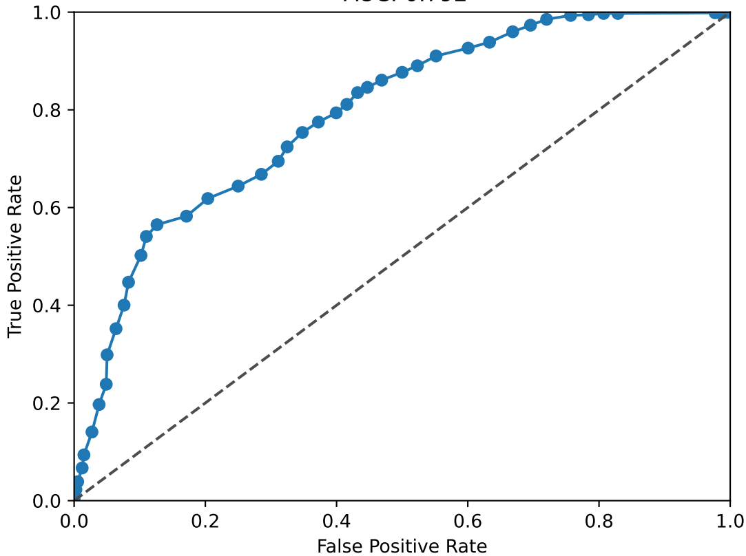
TBX15 ROC Curve AUC: 0.792
