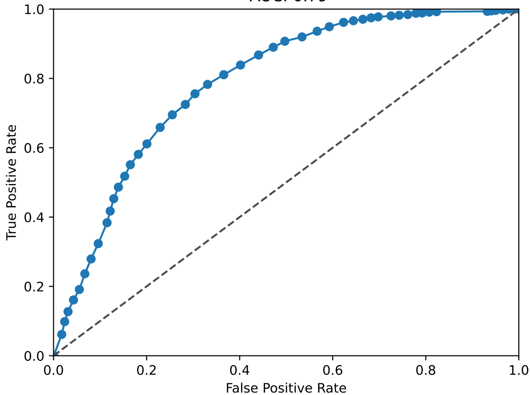
EGR1 ROC Curve AUC: 0.79
