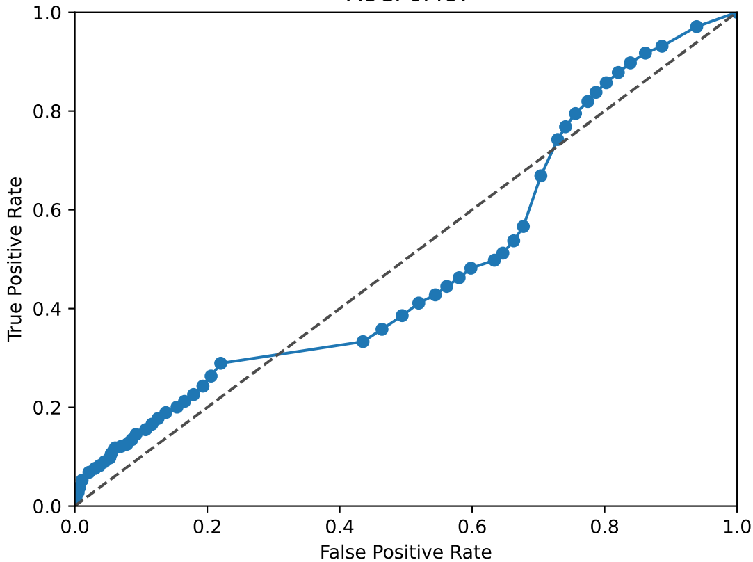
NFIX ROC Curve AUC: 0.487
