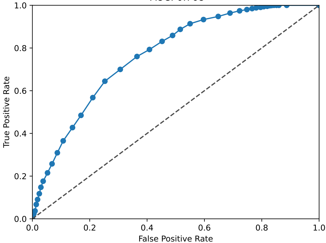
SIX4 ROC Curve AUC: 0.768
