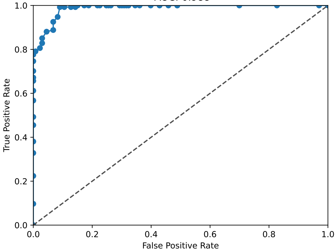
NFIB ROC Curve AUC: 0.988
