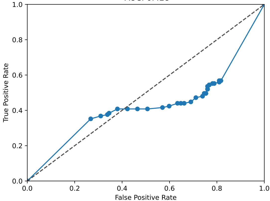
THR B ROC Curve AUC: 0.428
