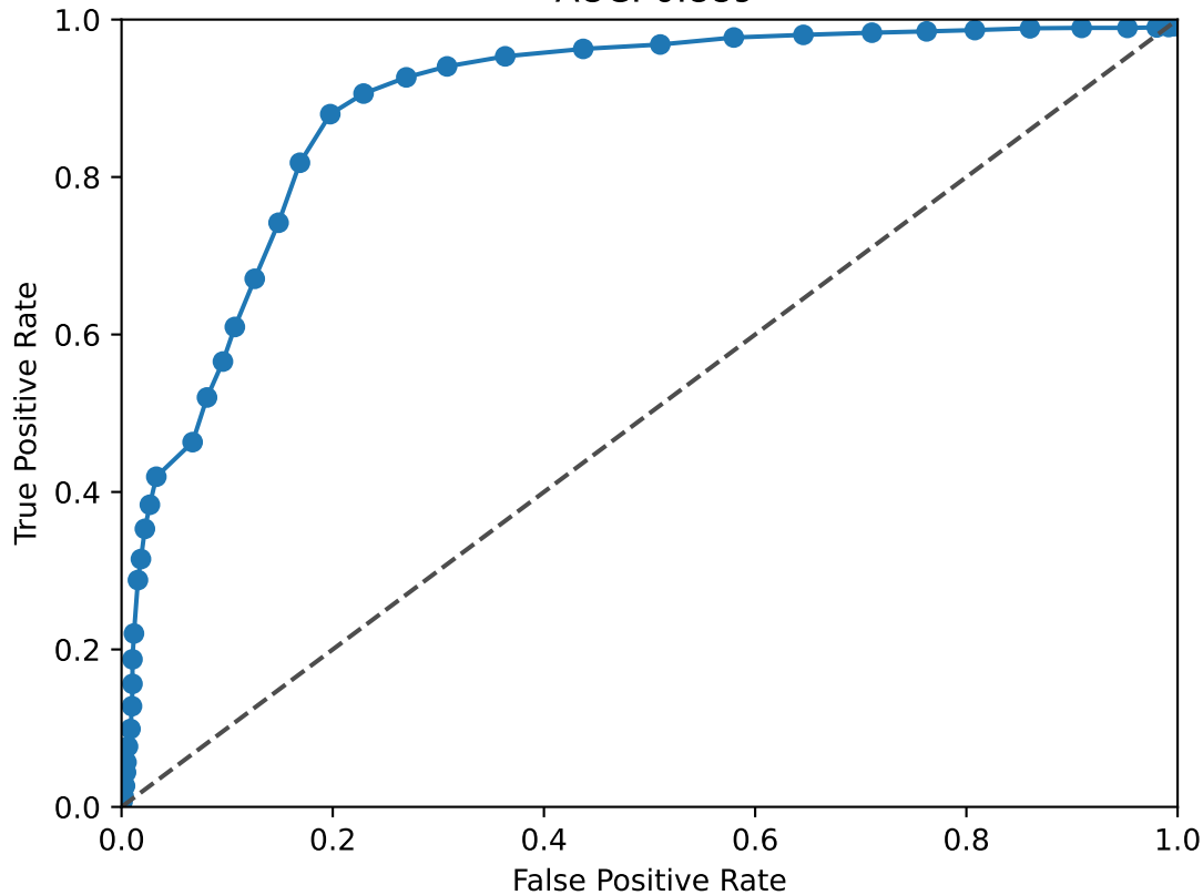
FOS ROC Curve AUC: 0.889
