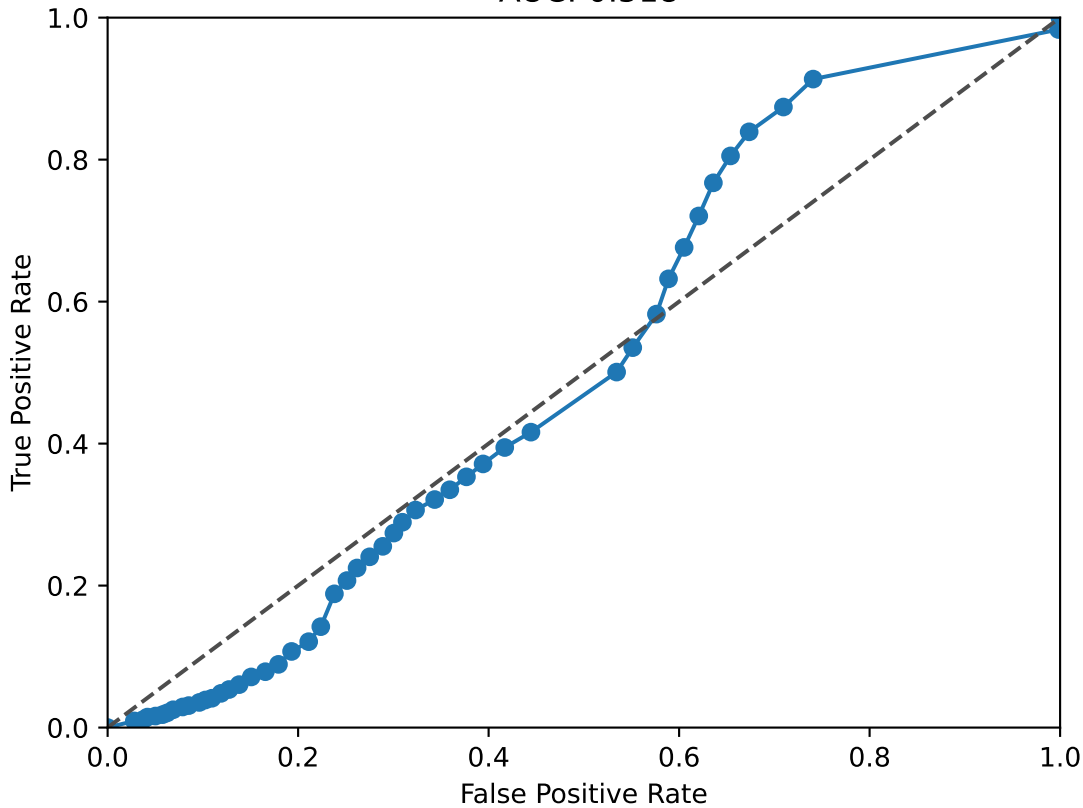
SIX1 ROC Curve AUC: 0.518
