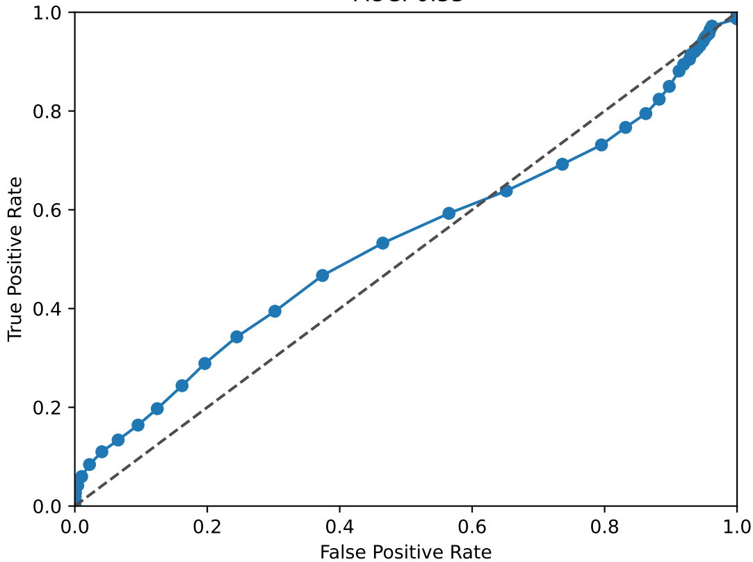
SIX4 ROC Curve AUC: 0.53
