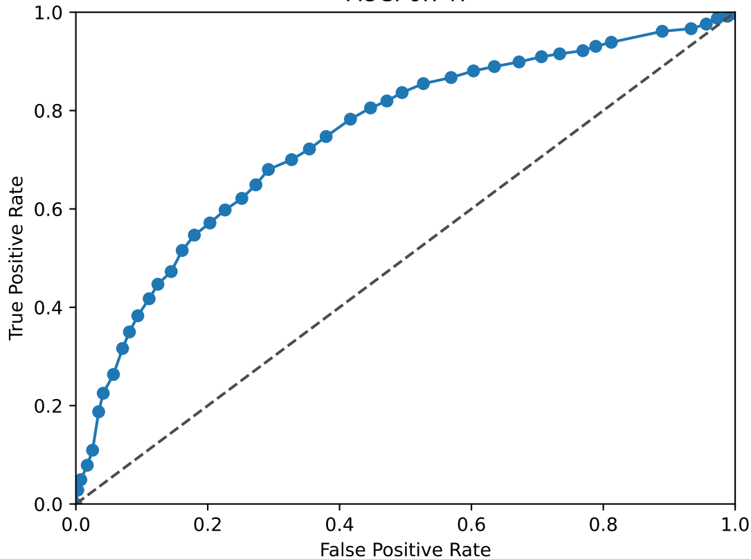
BACH1 ROC Curve AUC: 0.747
