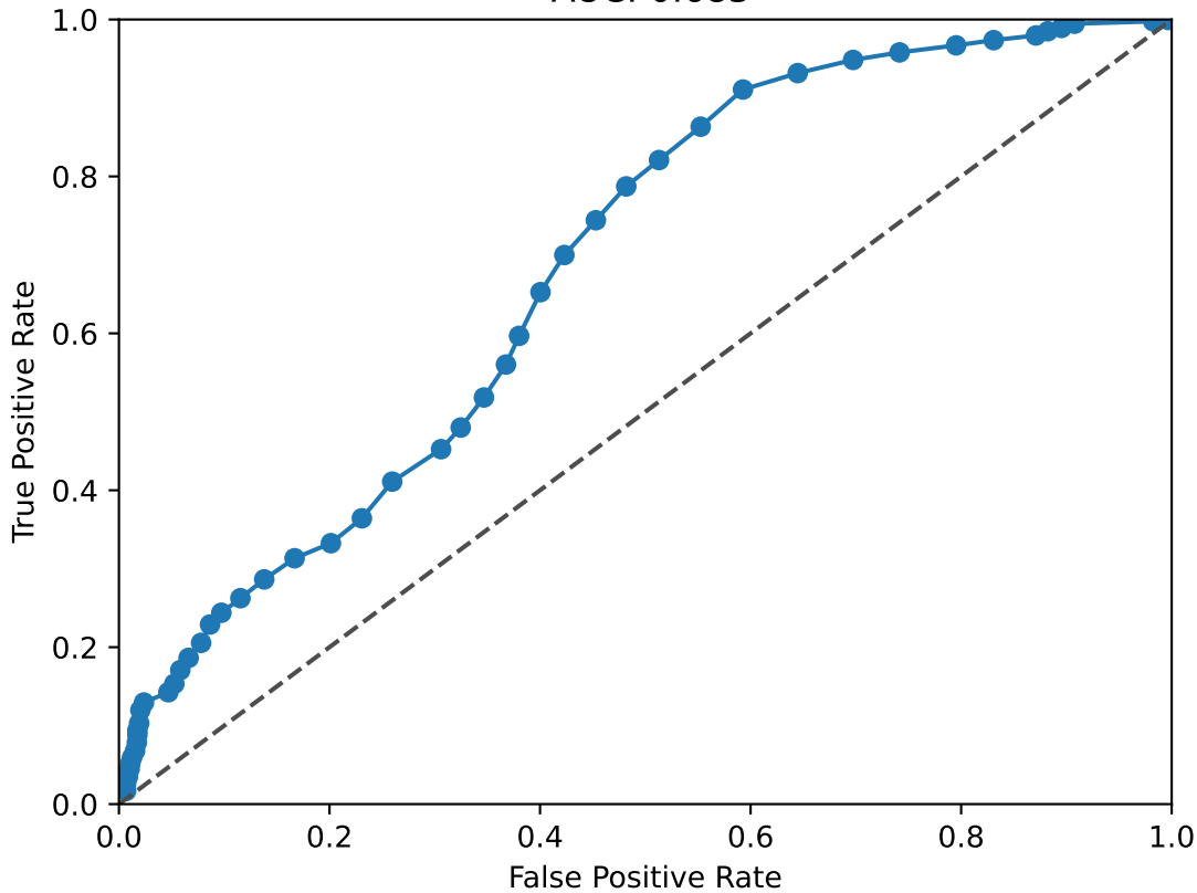
ICAM1 ROC Curve AUC: 0.683
