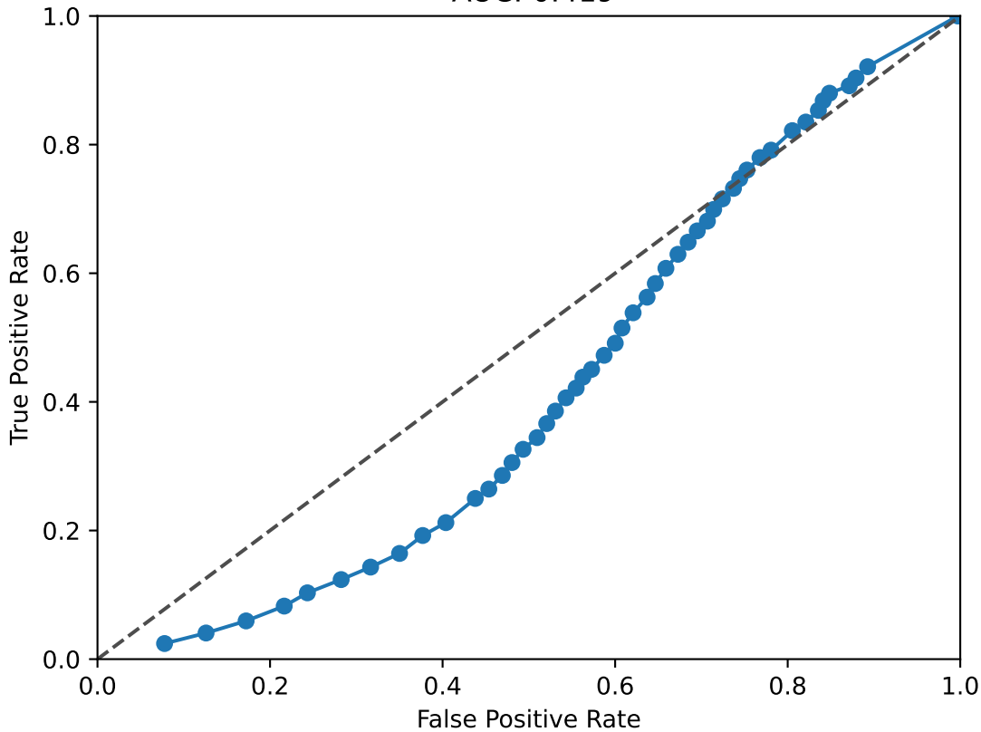
RORA_RORB ROC Curve AUC: 0.419
