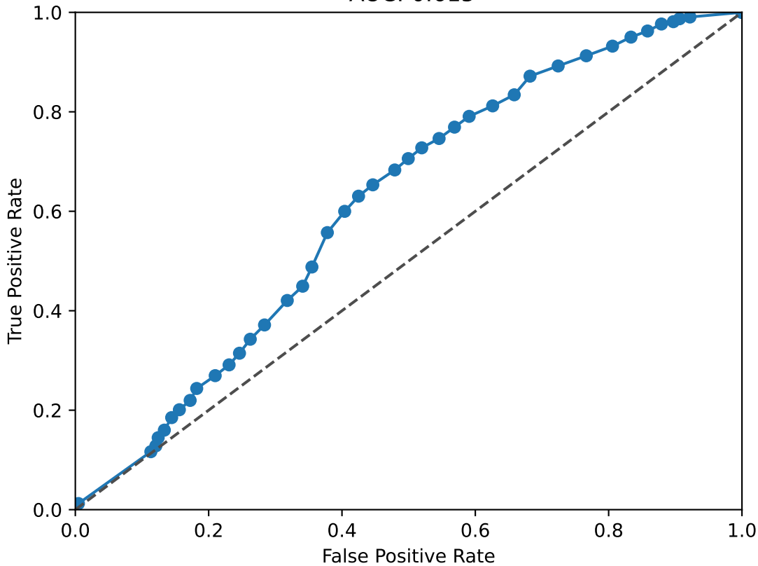
STAT2 ROC Curve AUC: 0.615
