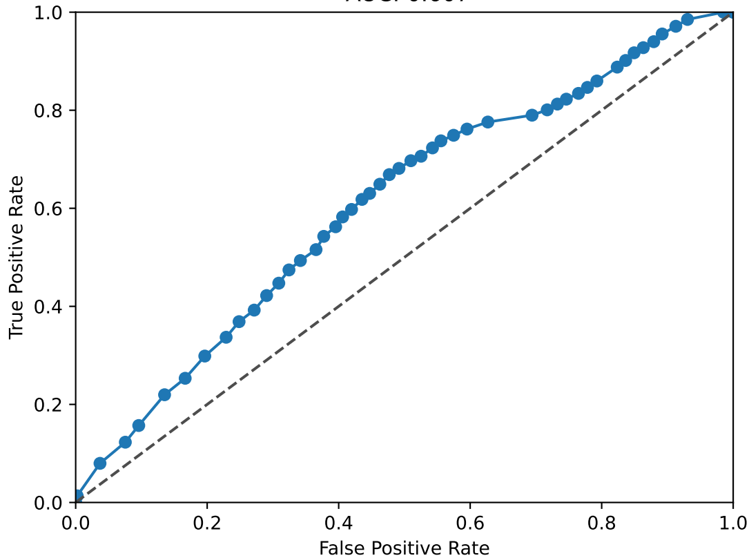
BACH1 ROC Curve AUC: 0.607
