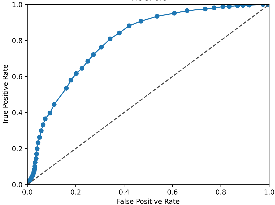
ICAM1 ROC Curve AUC: 0.8
