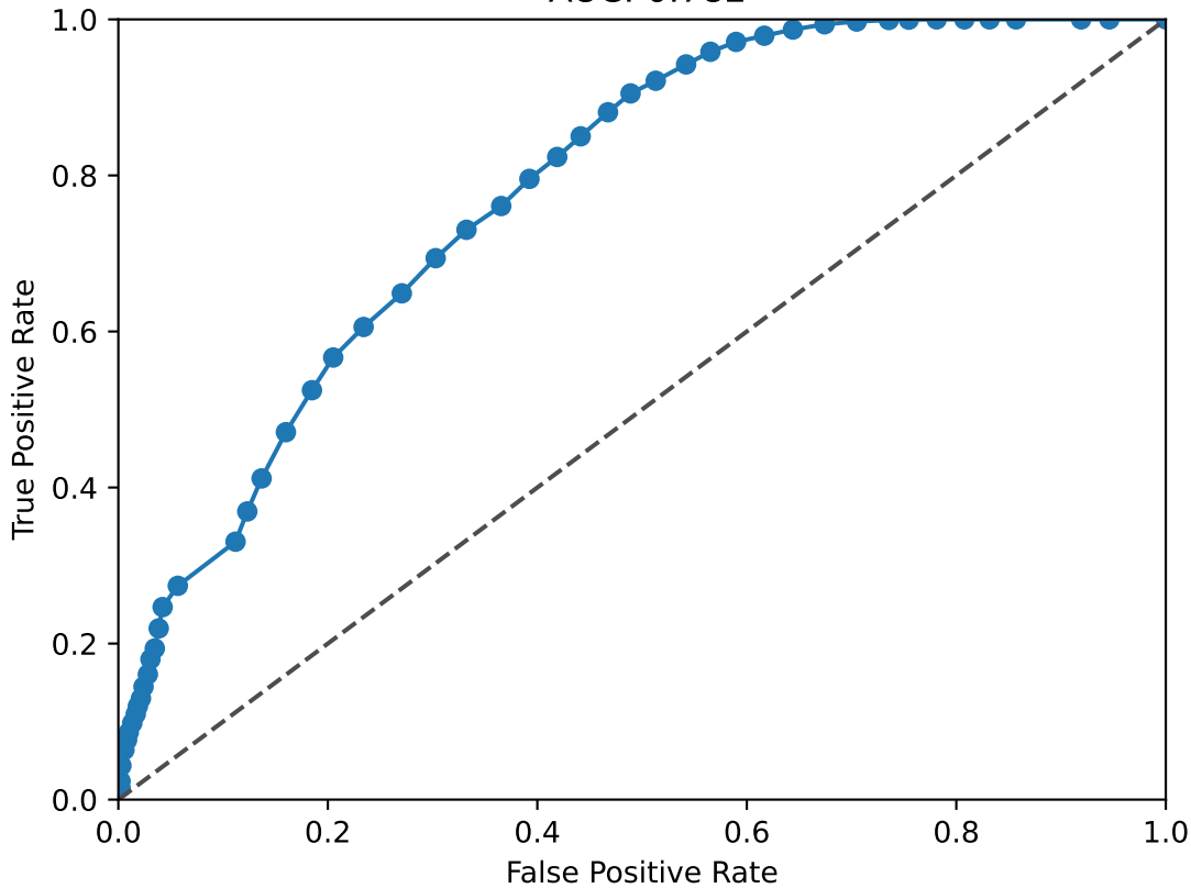
NFIA ROC Curve AUC: 0.782
