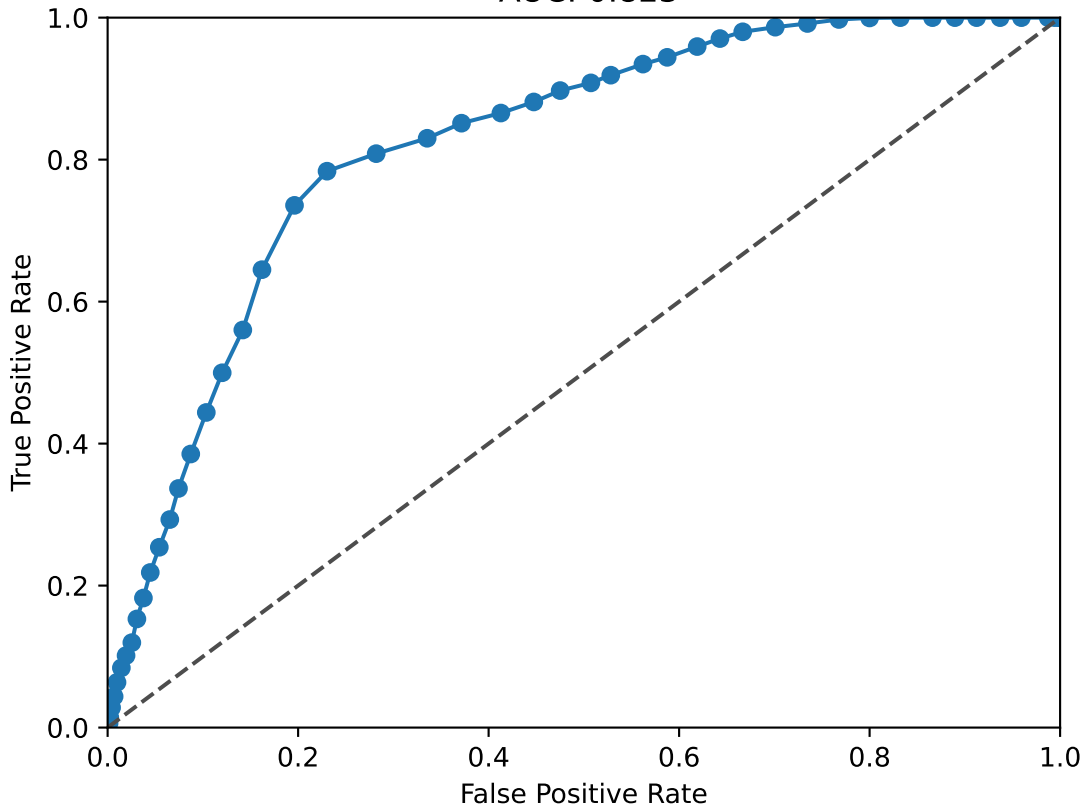
NFIB ROC Curve AUC: 0.823
