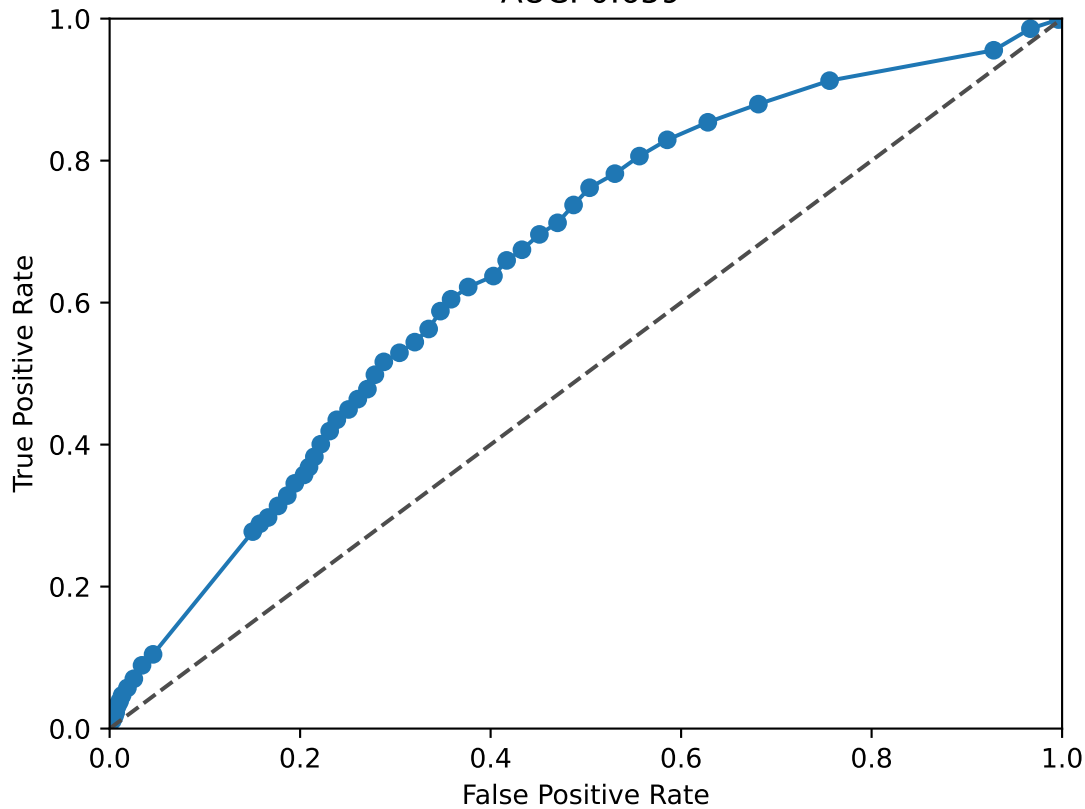
SMAD3 ROC Curve AUC: 0.659
