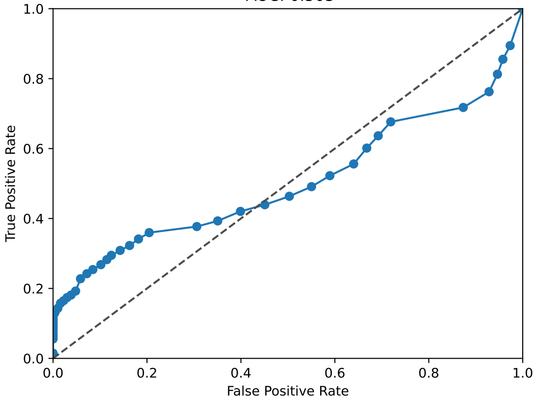
TCF7L2 ROC Curve AUC: 0.503
