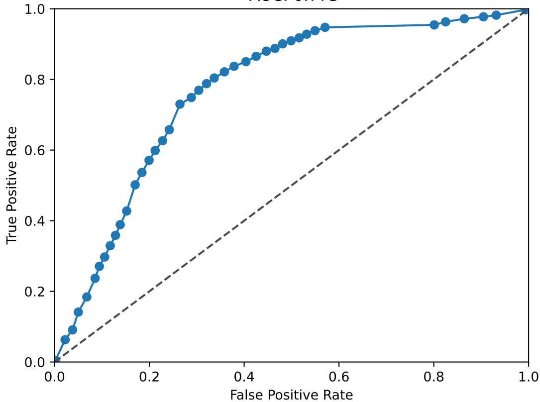
ETS1 ROC Curve AUC: 0.773
