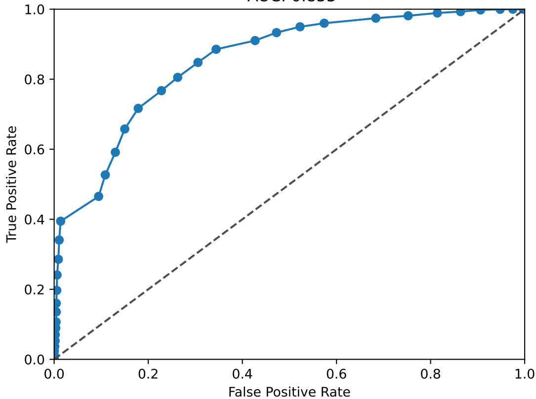
FOS ROC Curve AUC: 0.853
