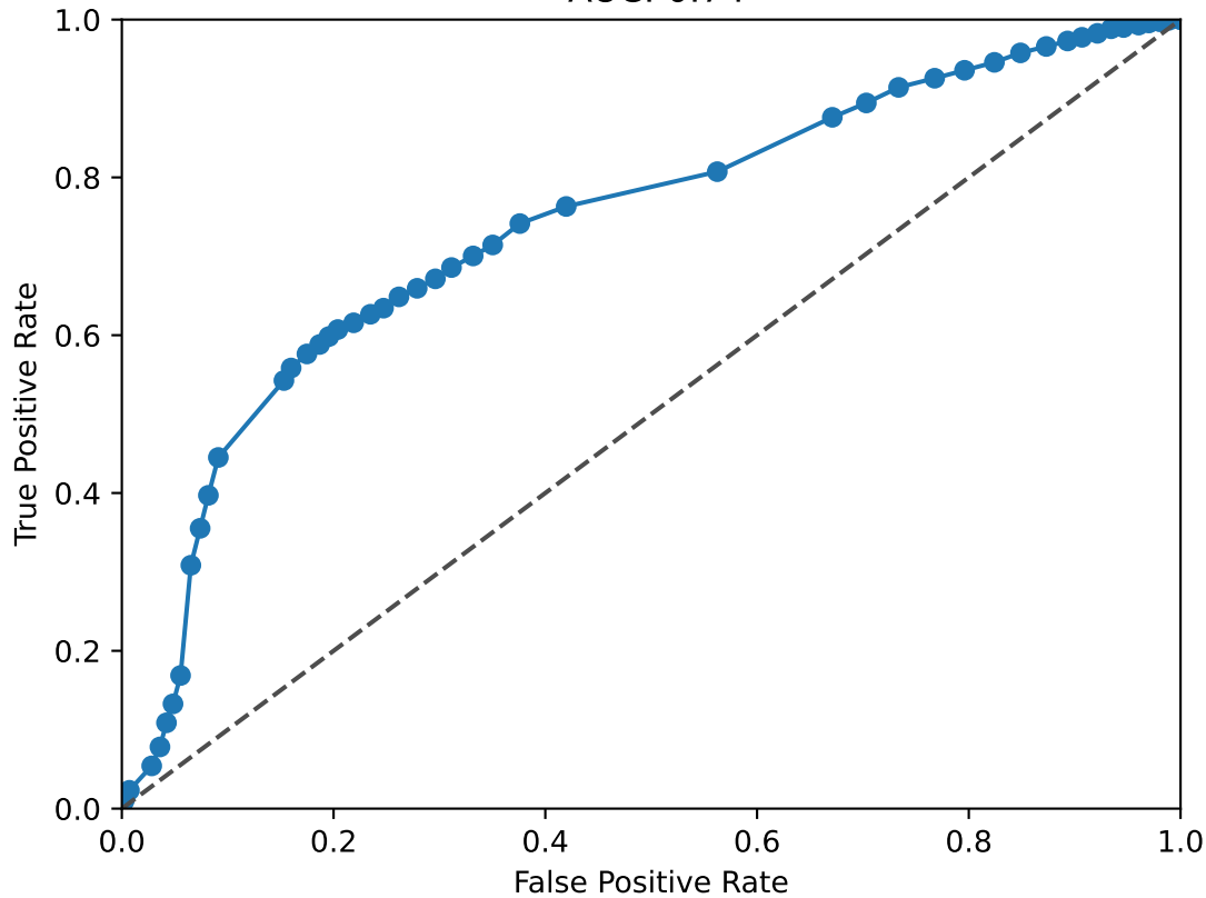
NFKB1 ROC Curve AUC: 0.74
