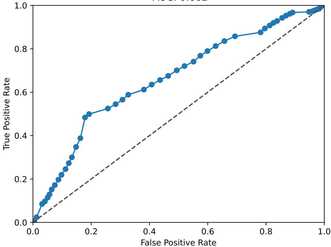
RORA_RORB ROC Curve AUC: 0.662
