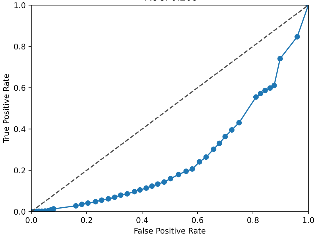
SOX11 ROC Curve AUC: 0.268
