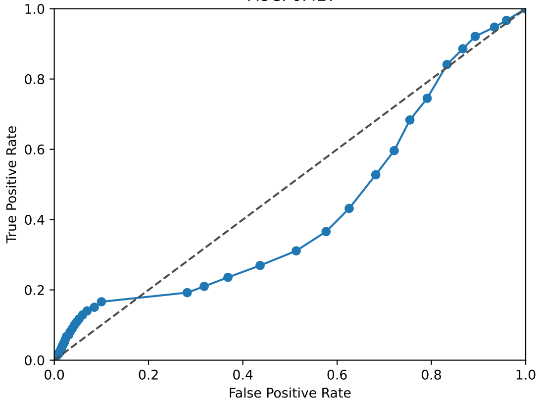
TCF7L2 ROC Curve AUC: 0.427
