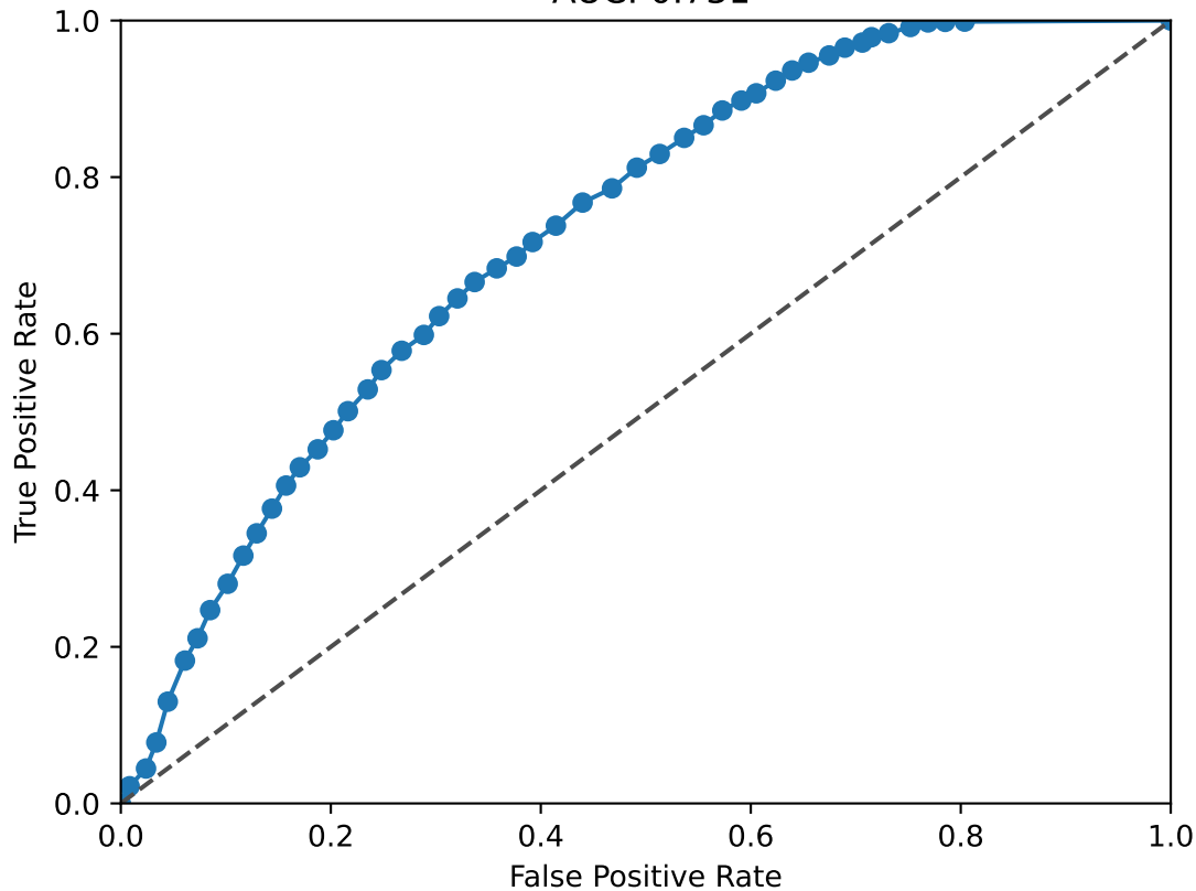
ZBTB20 ROC Curve AUC: 0.731
