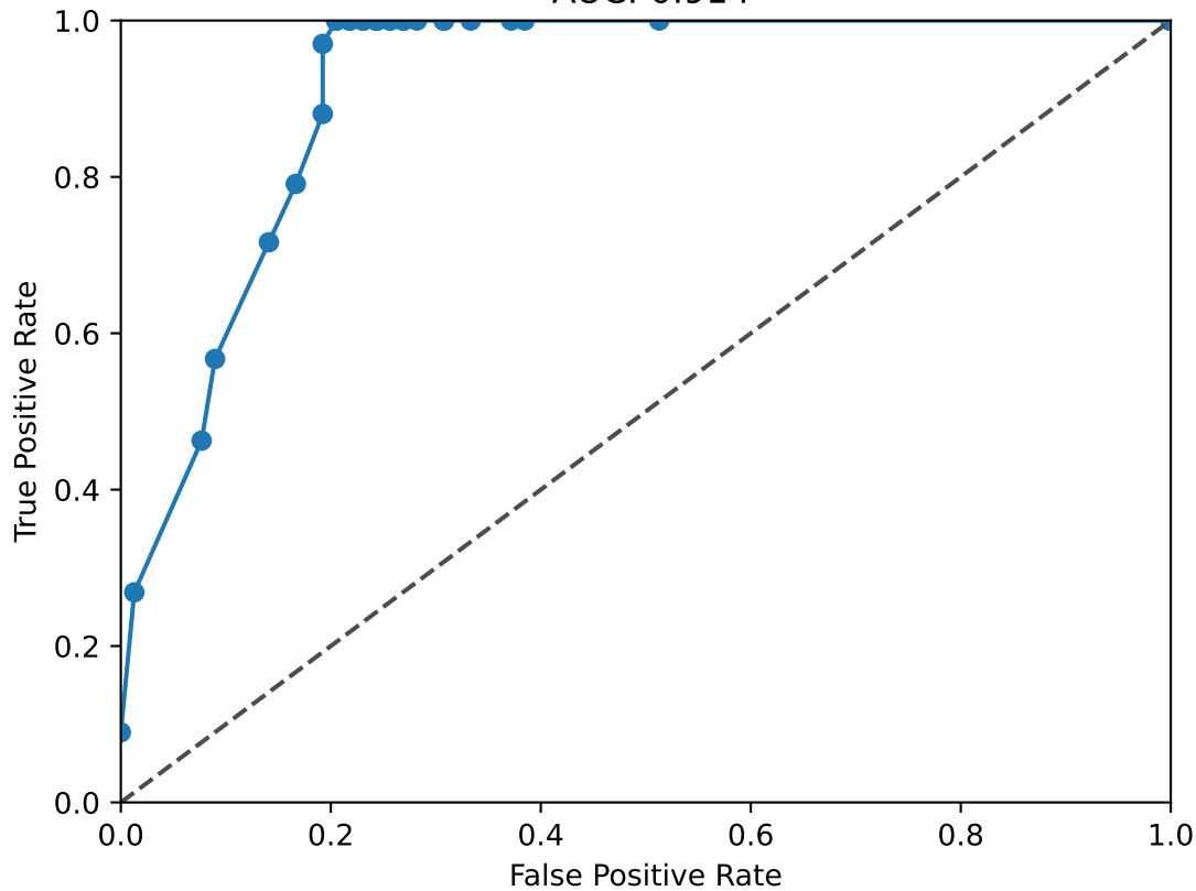
LMX1B ROC Curve AUC: 0.914
