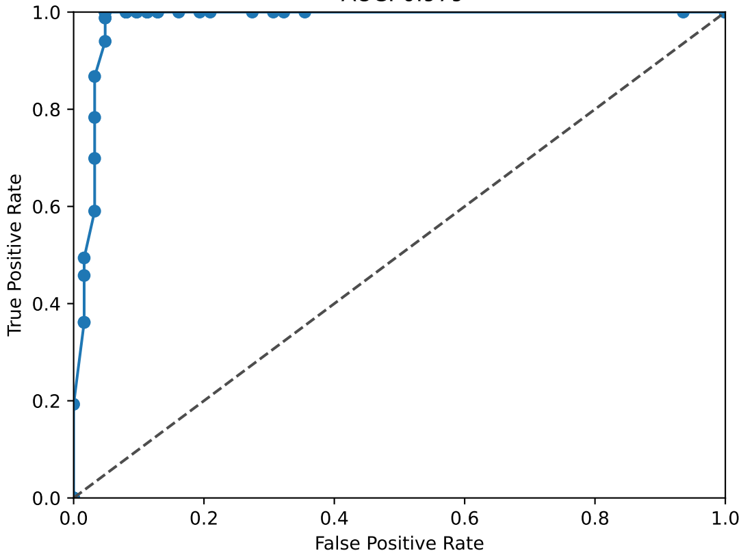
NFATC2 ROC Curve AUC: 0.979
