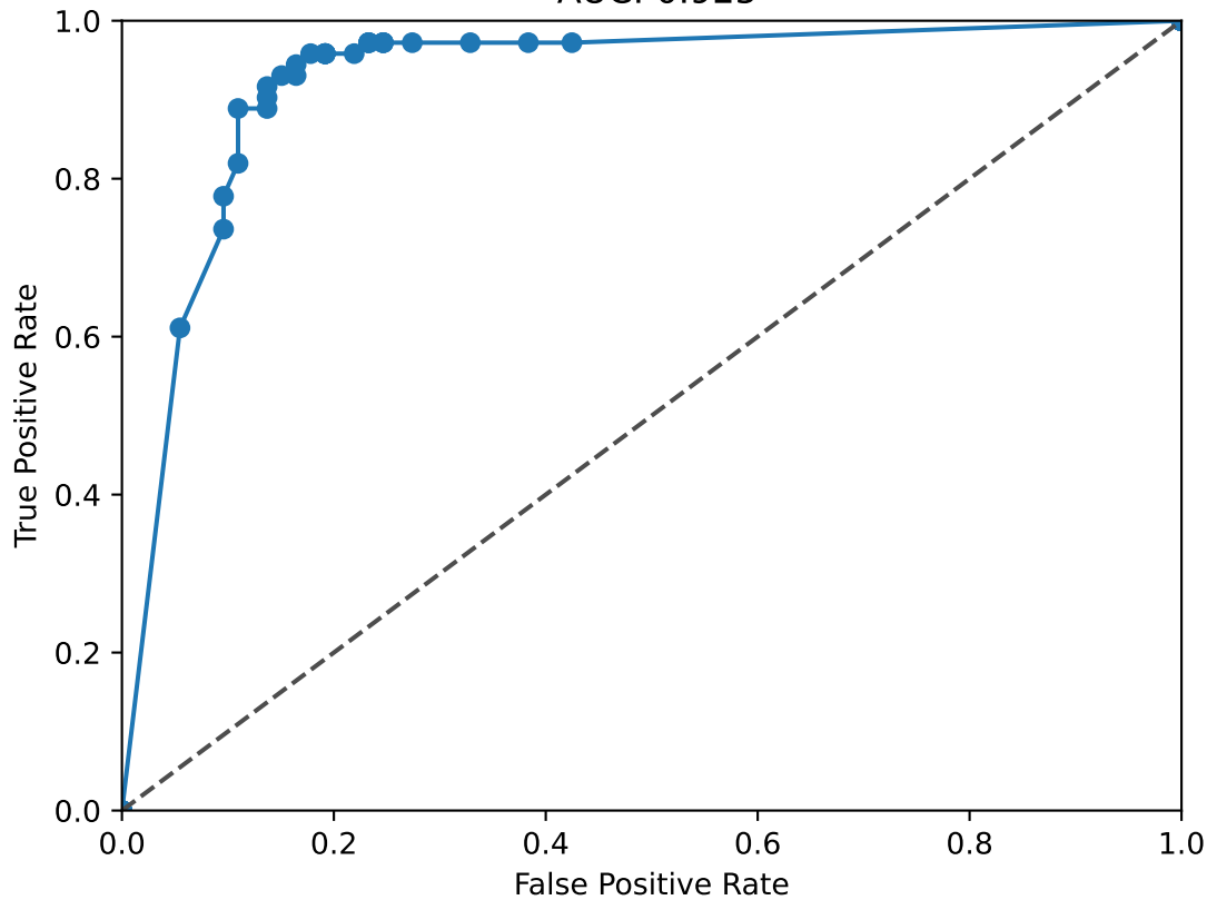
THRB ROC Curve AUC: 0.925
