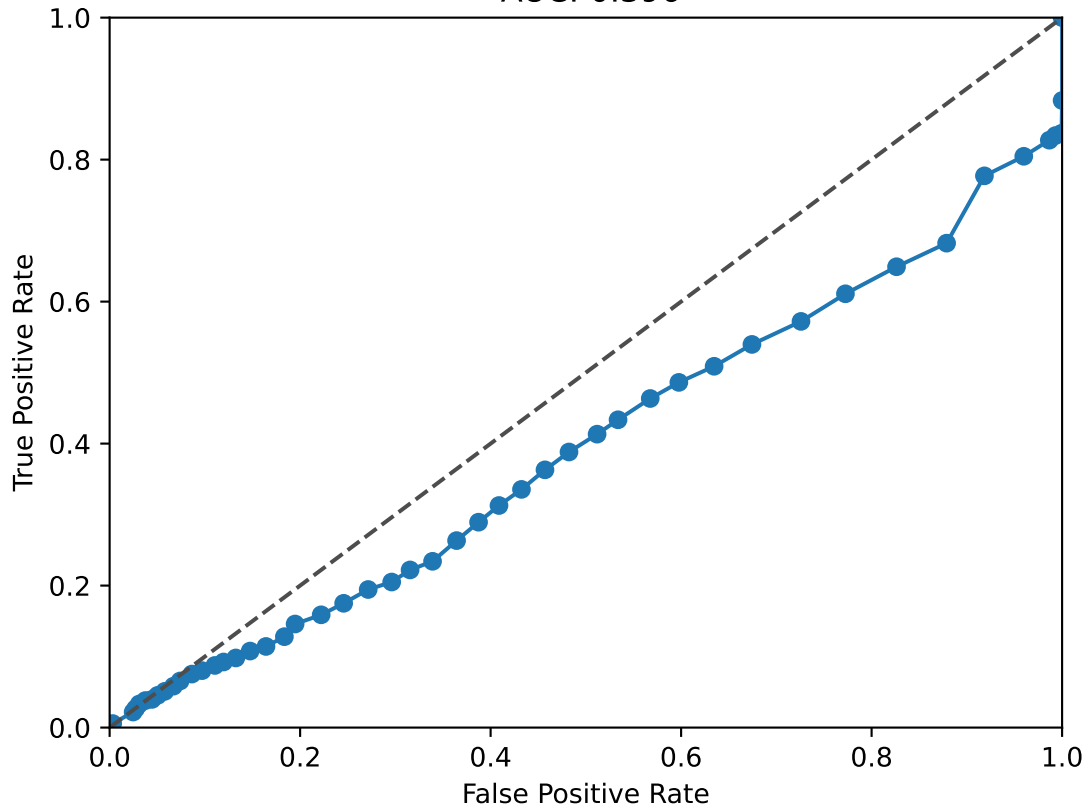
ASCL1 ROC Curve AUC: 0.396
