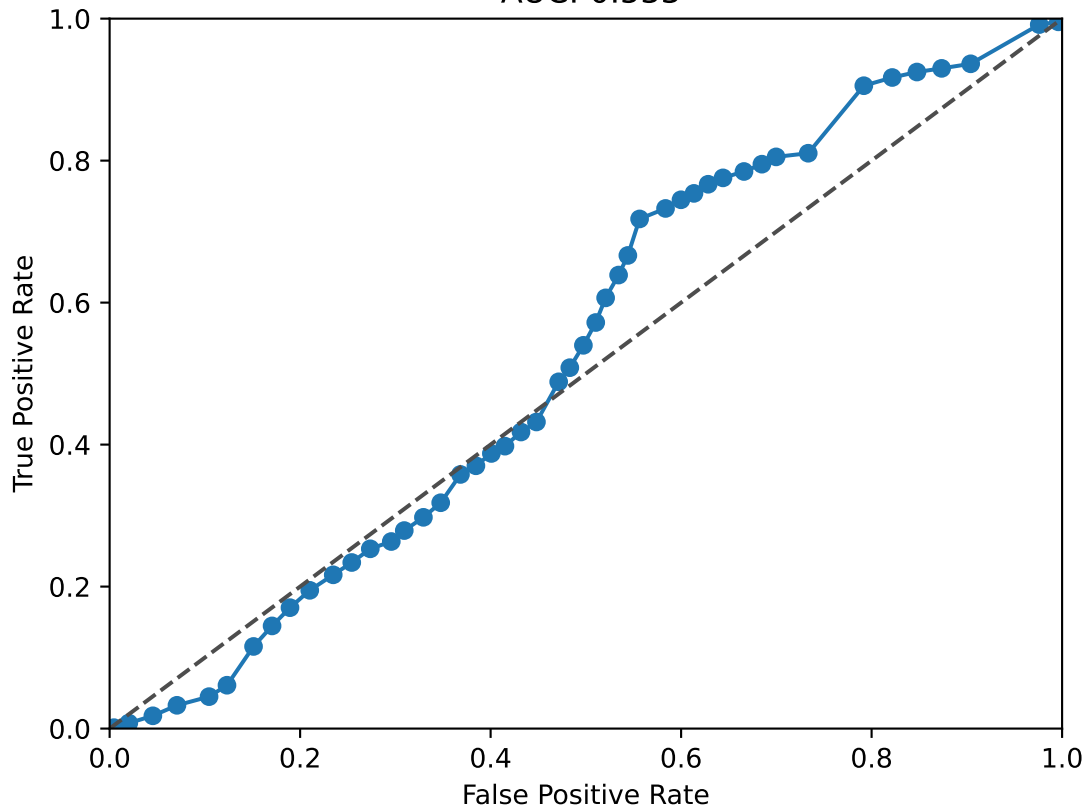
ETS1 ROC Curve AUC: 0.533
