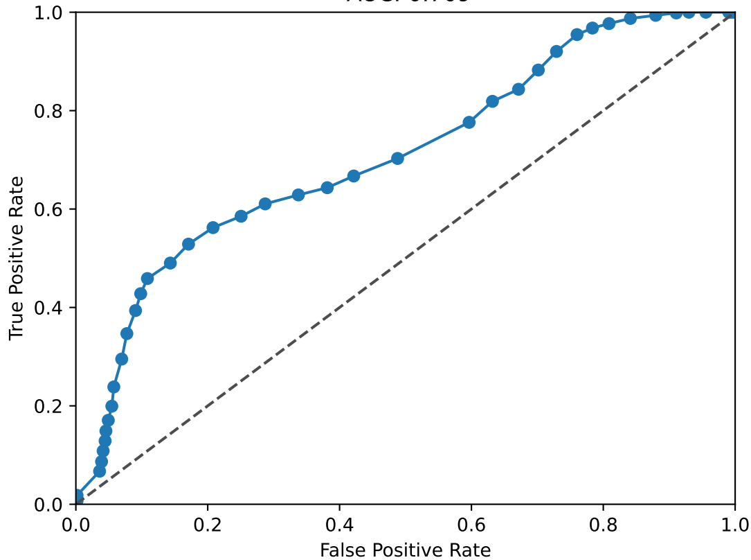
FOS ROC Curve AUC: 0.709
