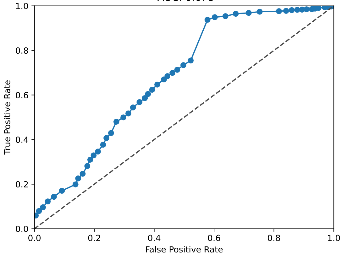
LMX1B ROC Curve AUC: 0.678
