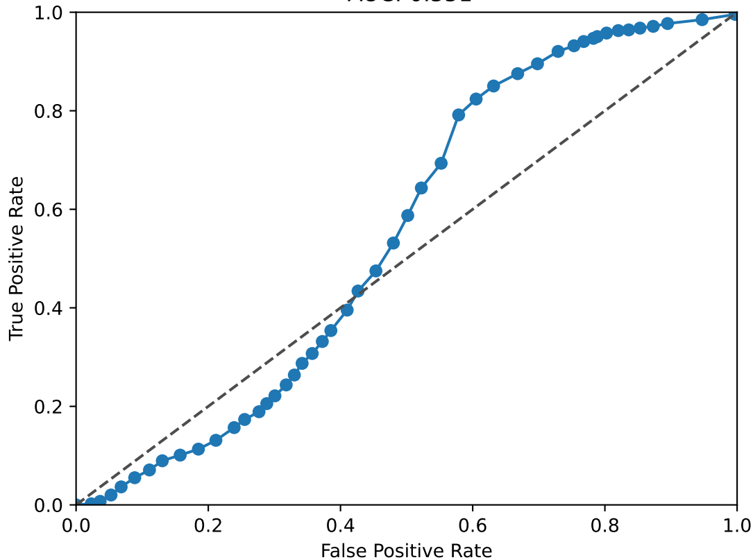
NCAM1 ROC Curve AUC: 0.551
