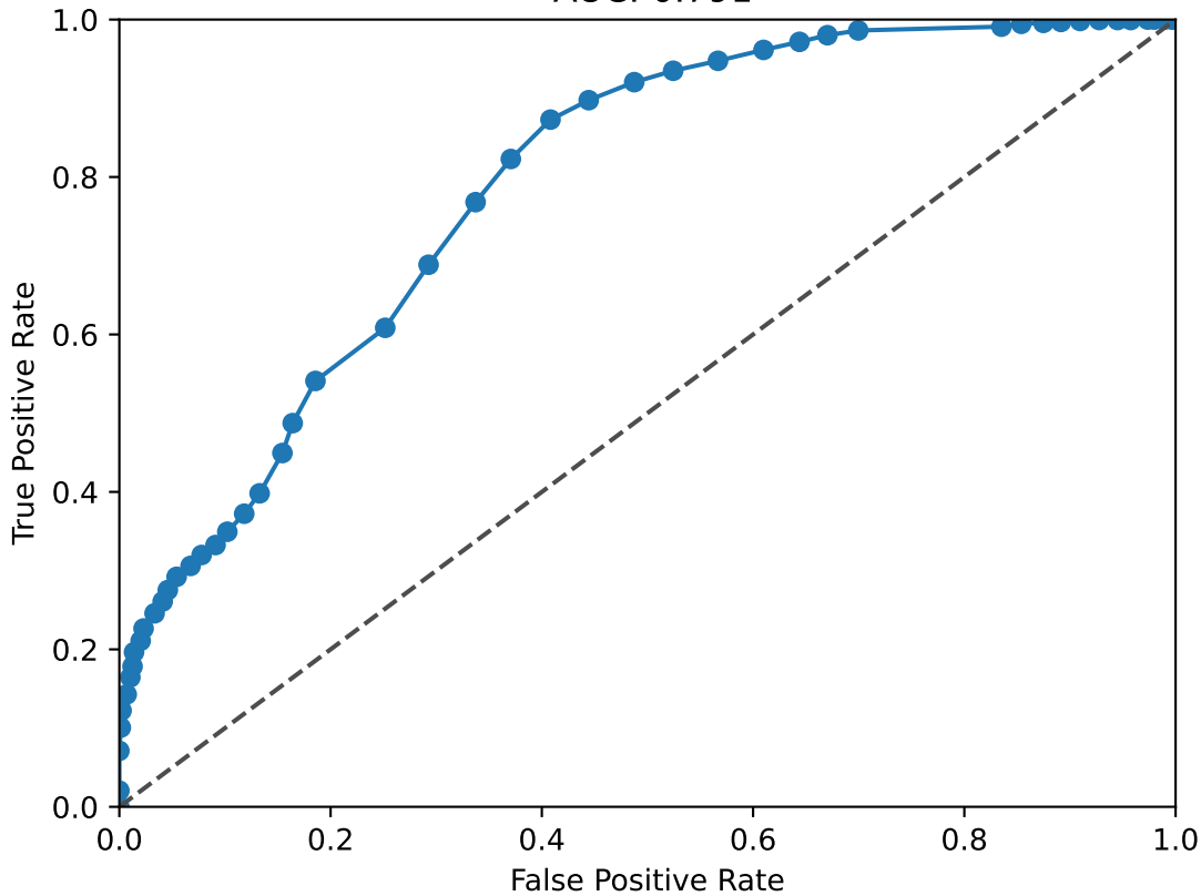
NFIB ROC Curve AUC: 0.791
