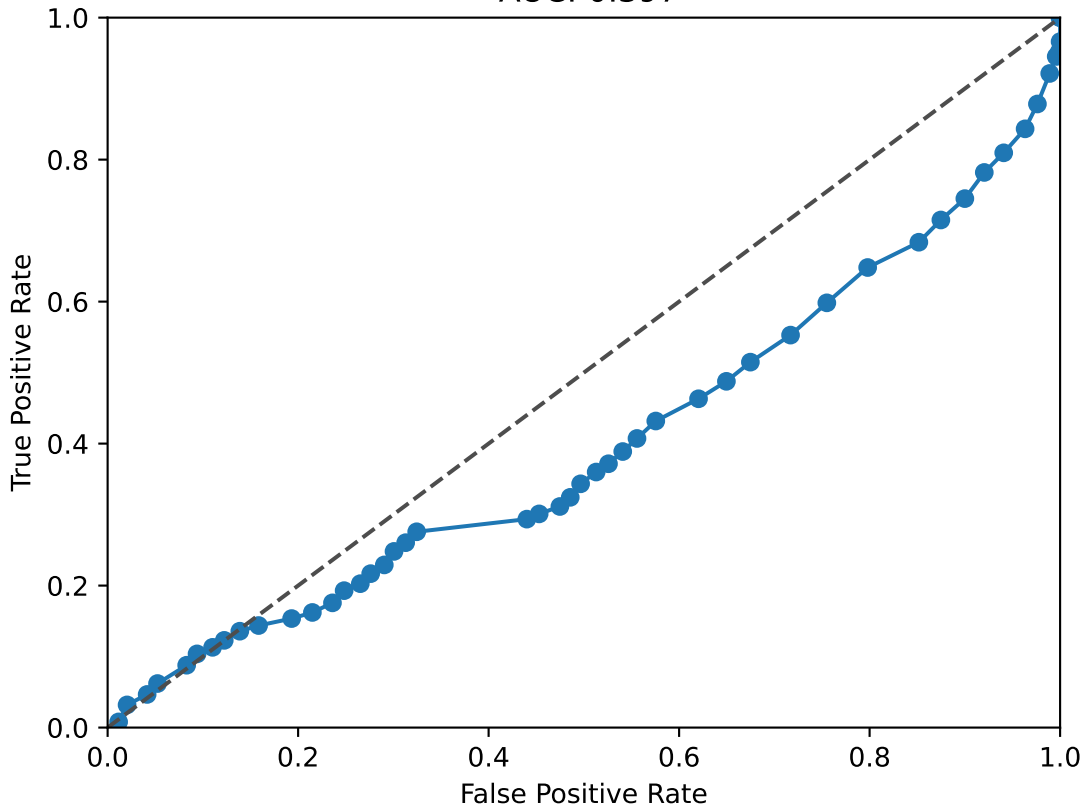
PKNOX2 ROC Curve AUC: 0.397
