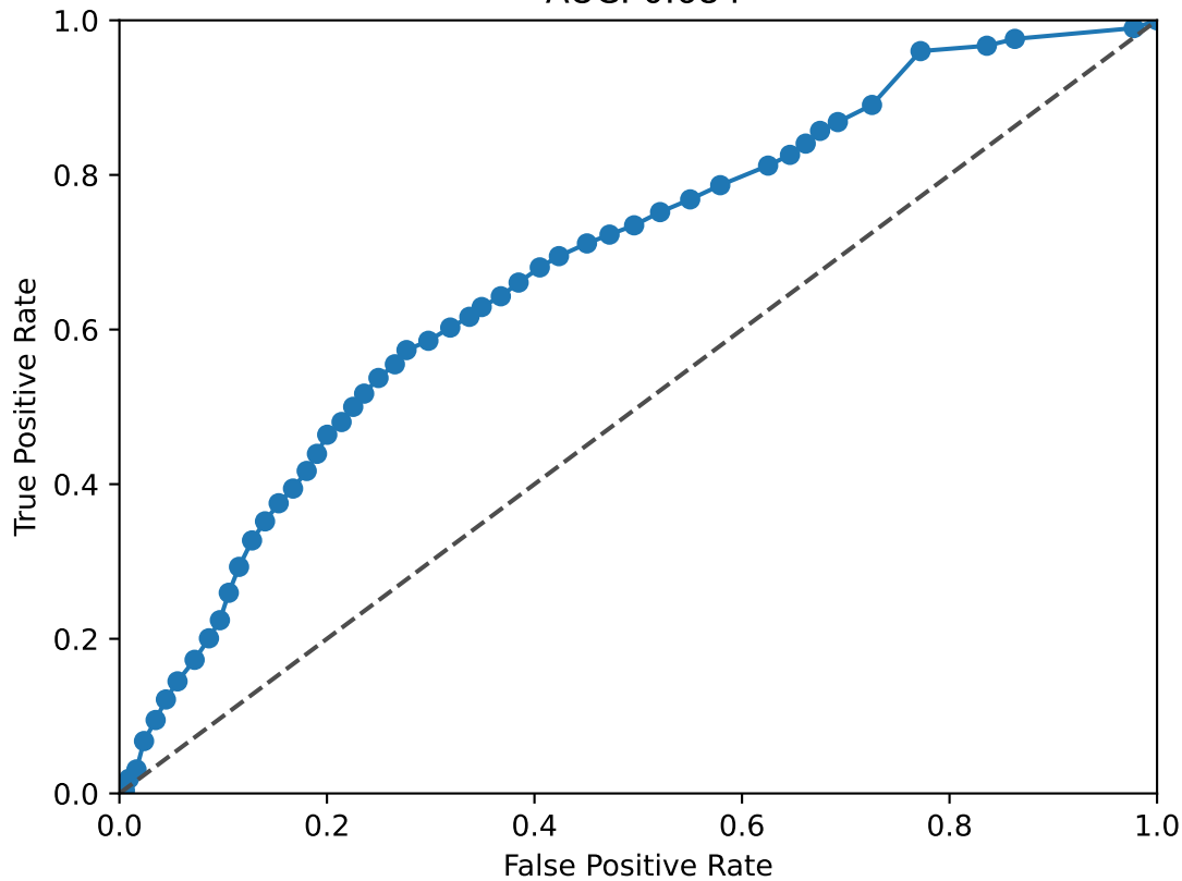
SMAD3 ROC Curve AUC: 0.684
