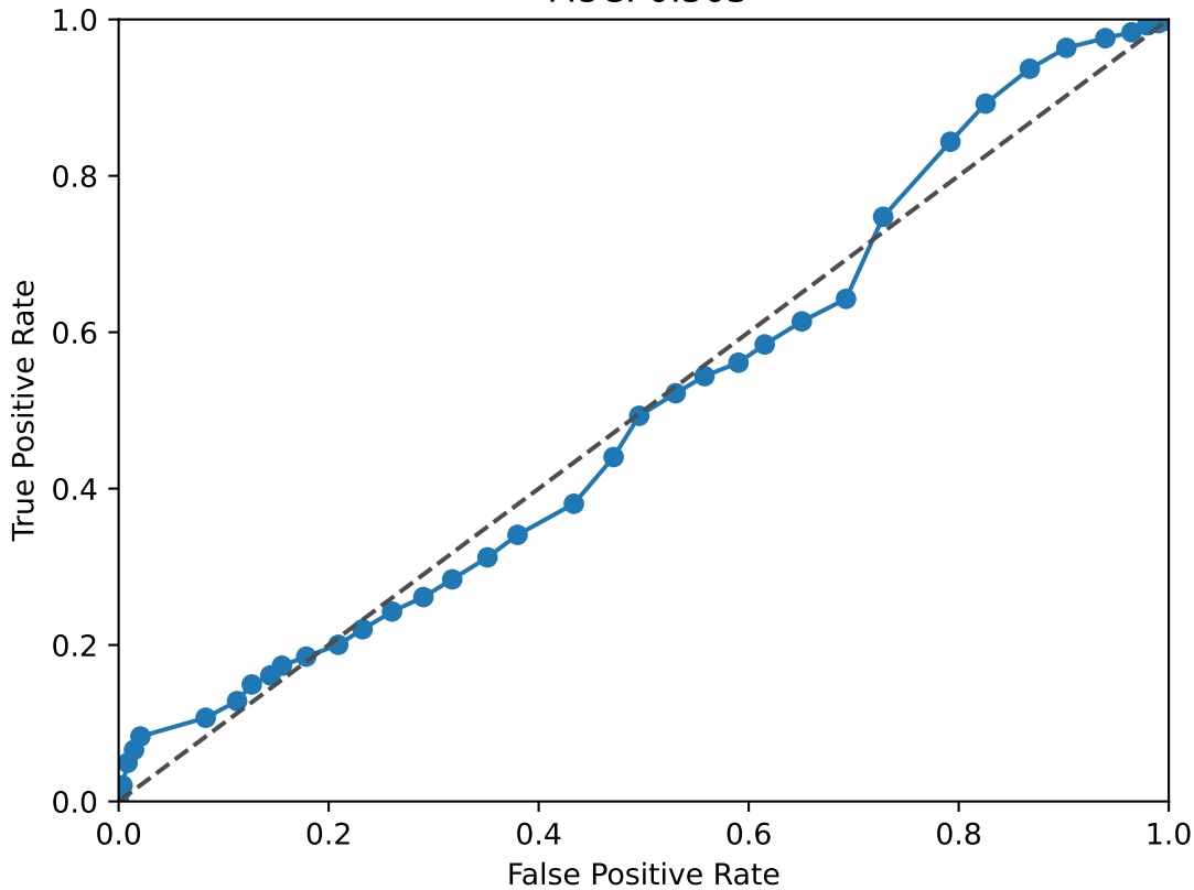
STAT2 ROC Curve AUC: 0.503
