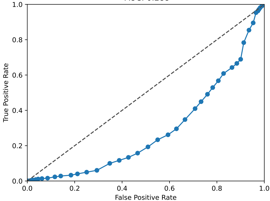
TCF7L1 ROC Curve AUC: 0.288
