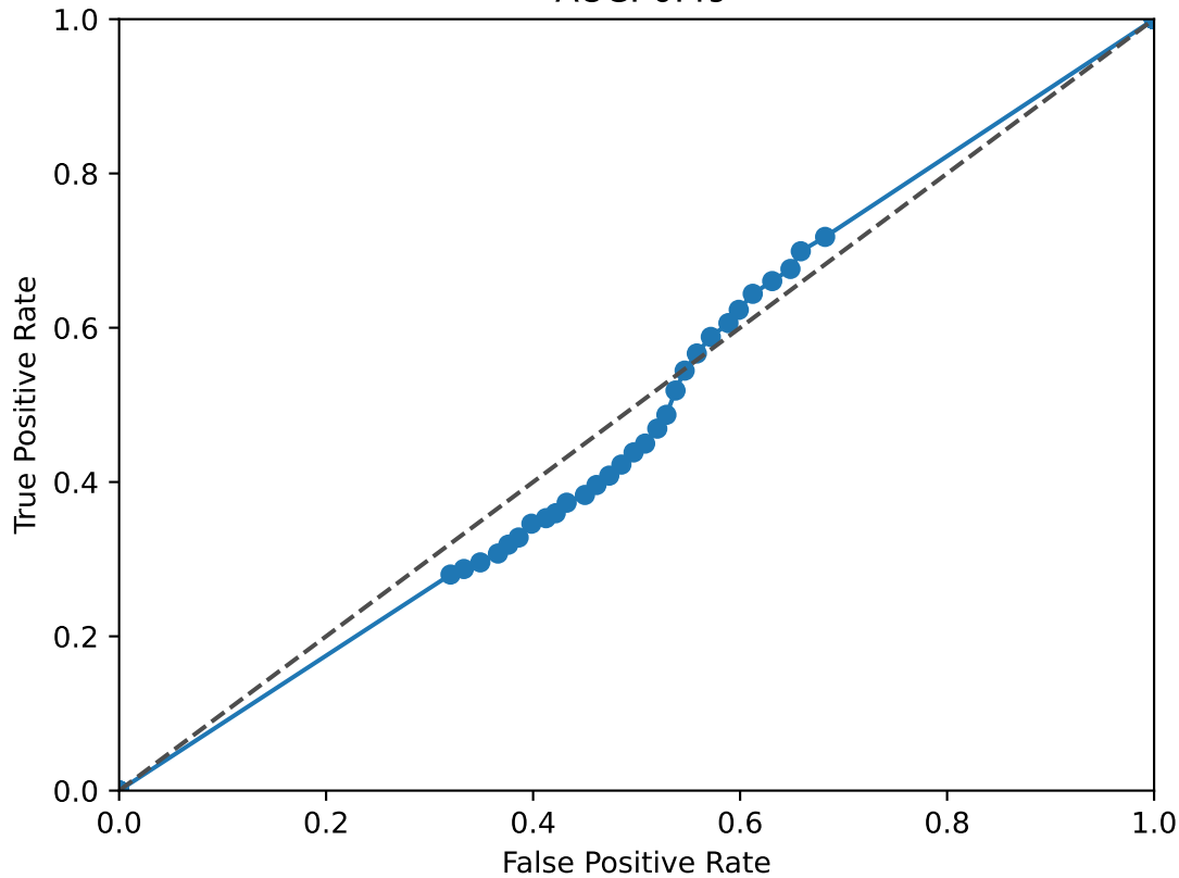
THR B ROC Curve AUC: 0.49
